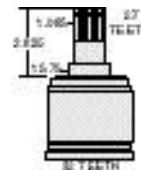
188-70L -INBOARD JOINT ASSEMBLY 1985-1989 Honda Accord 1985-1987 Honda Prelude
