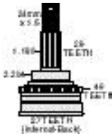
166-71B -OUTBOARD JOINT ASSEMBLY 1985-1994 Nissan Maxima Exc. DOHC 1987-1992 Nissan Stanza
